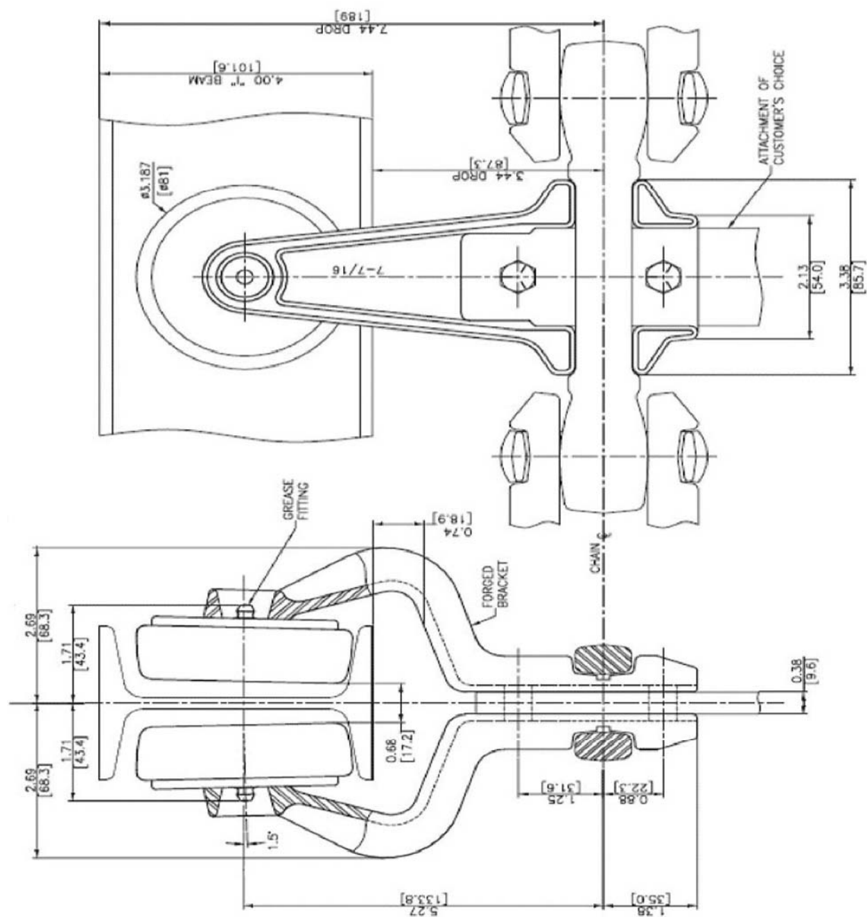
4" I-BEAM — TROLLEY X678 Chain — Vertical Hole — 7 7/16" (188.9) Drop
